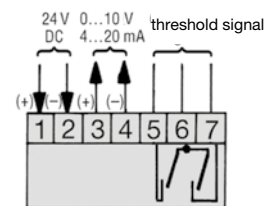
electrical connection
